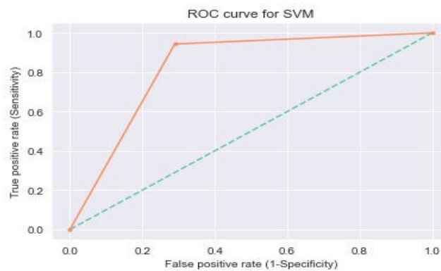
Figure 5: ROC Curve for SVM
