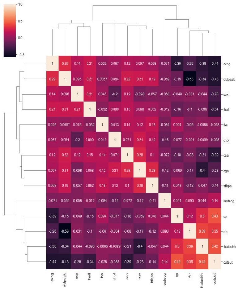
Figure 2: The Cluster Plot
