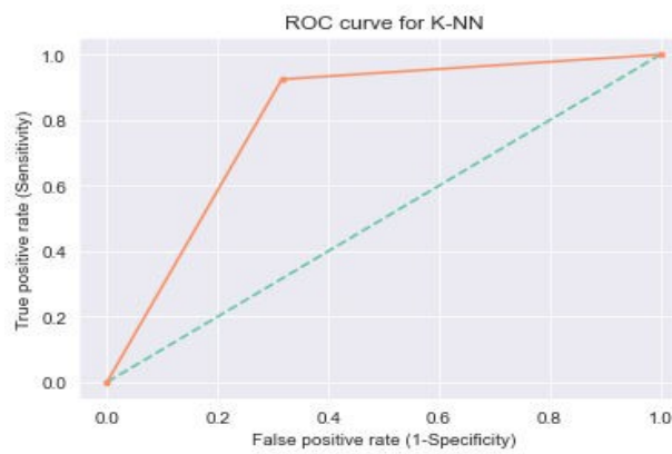
Figure 4: ROC Curve for K-NN
