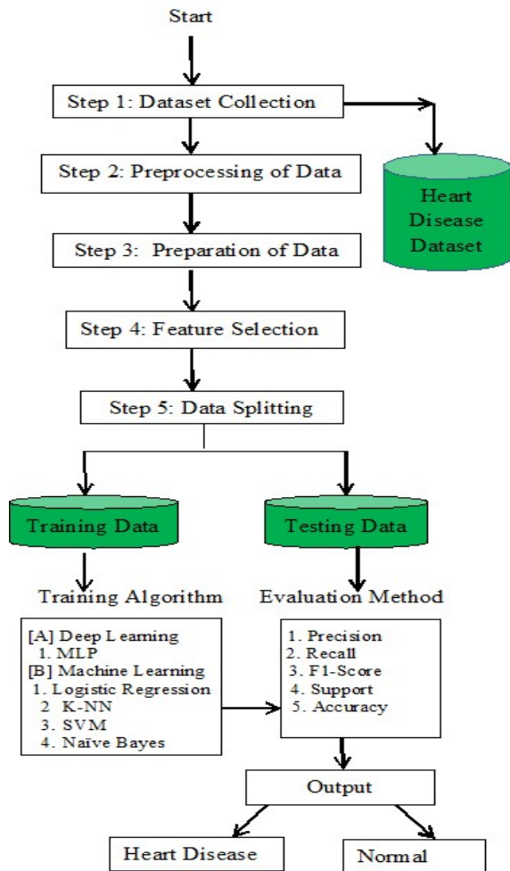
Figure 1: Flowchart for proposed system
