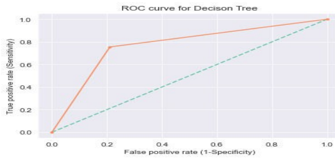
Figure 7: ROC Curve for Decision Tree
